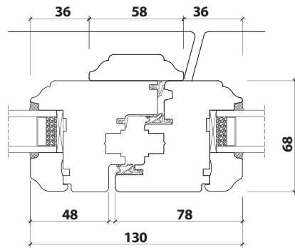
MENEAU STANDARD
